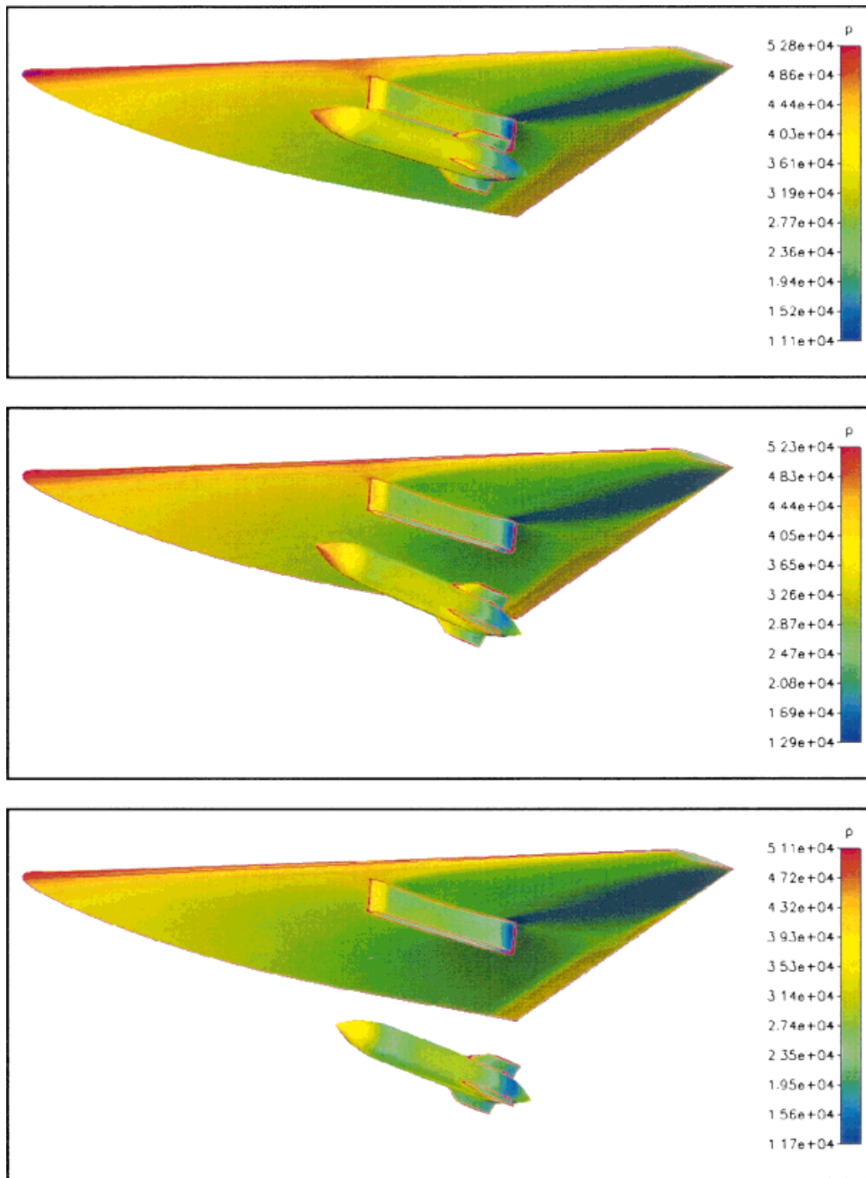
Plate 3. Pressure contours on the surface of the delta wing and the store body and t = 0 s, t = 0.191 s and t = 0.32 s. Inviscid solution corresponds to a free-stream Mach number of 0.95 and angle of attack of 0.0^\circ .
